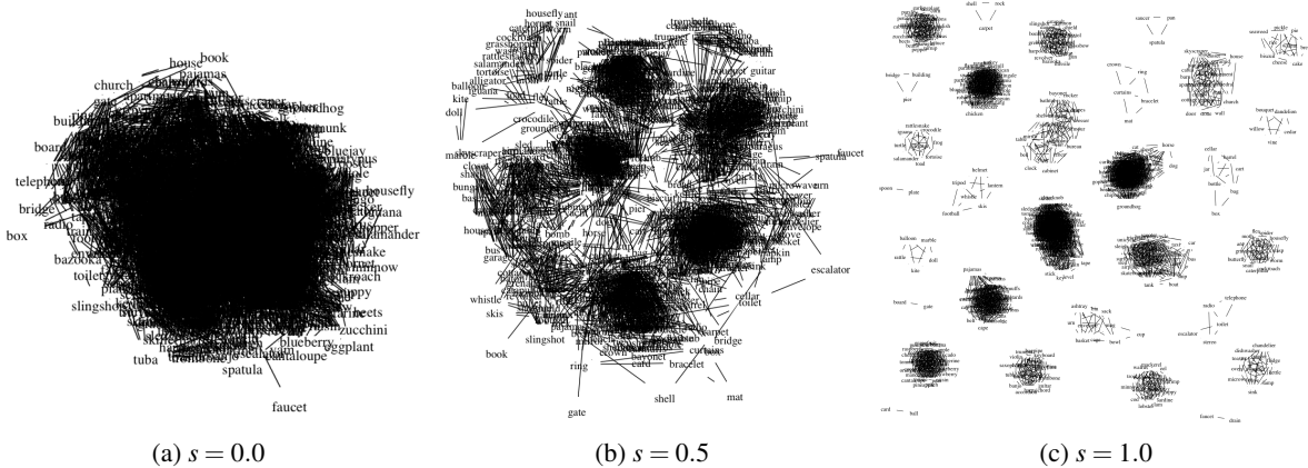
Figure 3: The original semantic network as derived from the BNC (a) and the same network re-weighted using a flat clustering produced by CW (b). As s approaches 1.0 the network exhibits an increasingly strong small-world property, eventually reconstructing the input clustering only (c).
